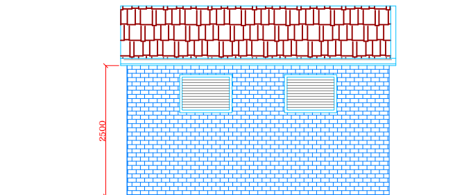
REFUSE STORE B REAR ELEVATION SCALE: 1/100
