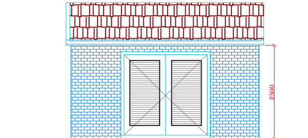
REFUSE STORE B FRONT ELEVATION SCALE: 1/100
