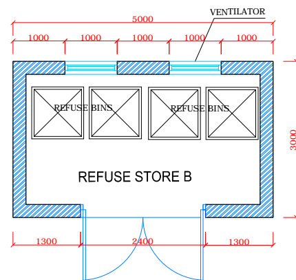
REFUSE STORE B FLOOR PLAN SCALE: 1/100
