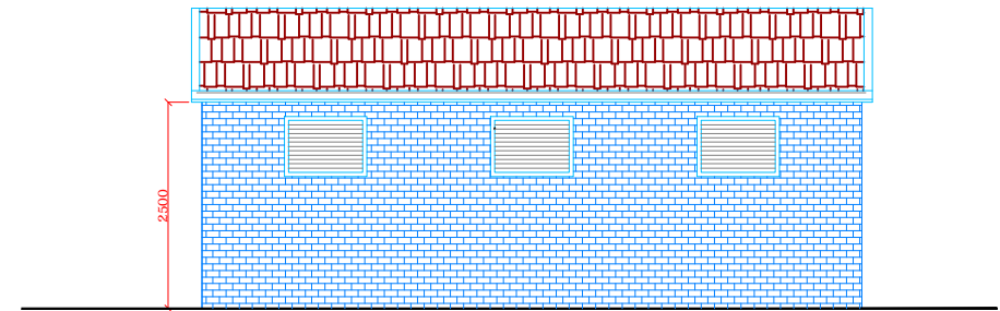
REFUSE STORE A REAR ELEVATION SCALE: 1/100
